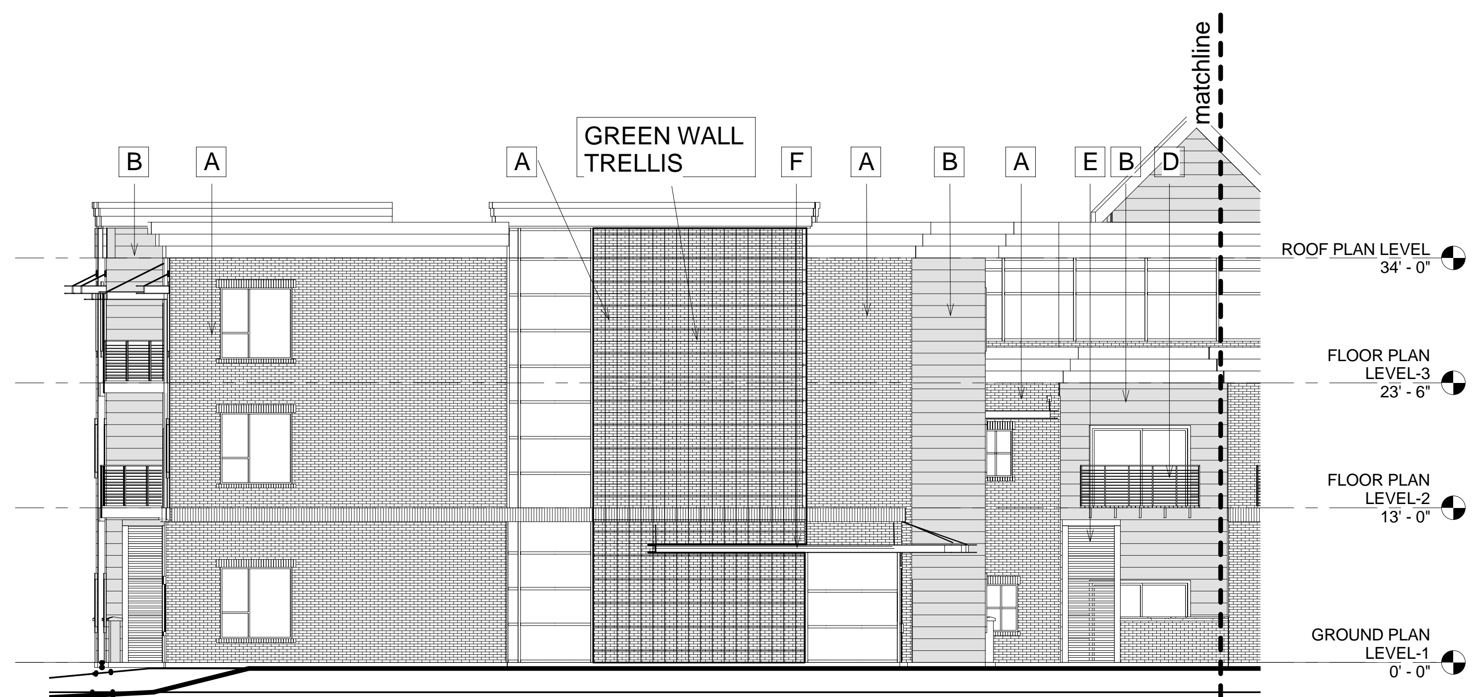
② BUILDING 1 PARTIAL ELEVATION NORTH 1/8" = 1'-0"
