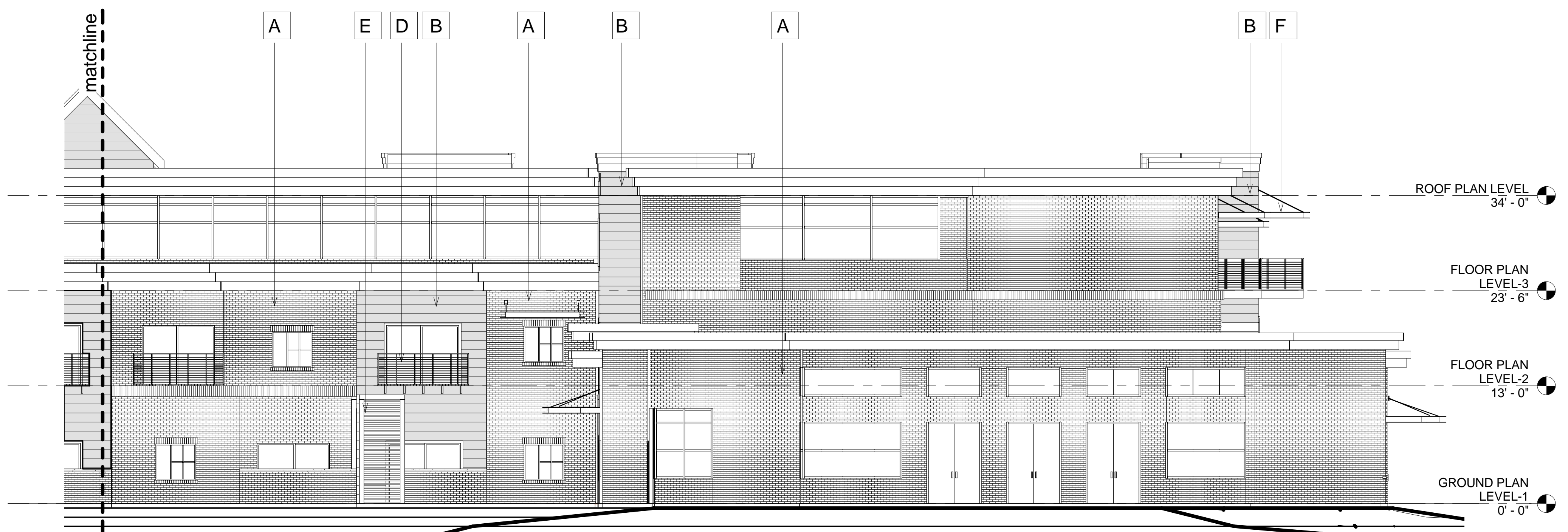
① BUILDING 1 ELEVATION NORTH 1/8" = 1'-0"
